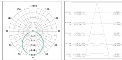
20W 60cm Surface Mounted Fixture
